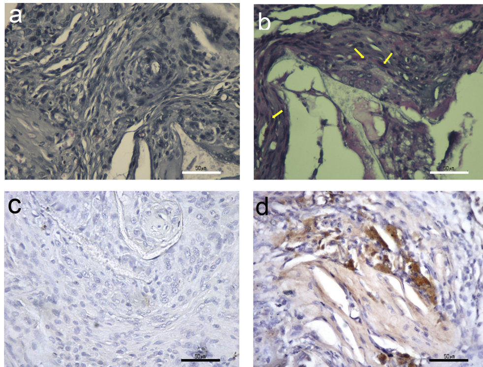
Fig. 5. Histological analysis of the graft site on the small bowel mesentery of the placebo group (a, c) and of the IMI group (b, d). Gomori staining (a, b) and insulin immunohistochemistry staining (c, d). Beta cells are indicated by yellow arrows (b) and insulin-positive cells stained in brown (d) 4-months post implantation, magnification 40 \times . Scale bar is 50 \mu m in all panels.
