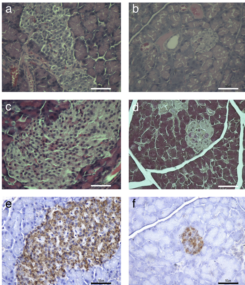
Fig. 4. Histological analysis of islet of Langerhans on non-treated rats (a, c, e) and on STZ-induced diabetic rats (b, d, f); HE staining in panels a and b. Gomori staining in panels c and d. Insulin immunohistochemistry staining in panels e and f. Magnification 40 \times . Scale bar is 50 \mu m in all panels.
